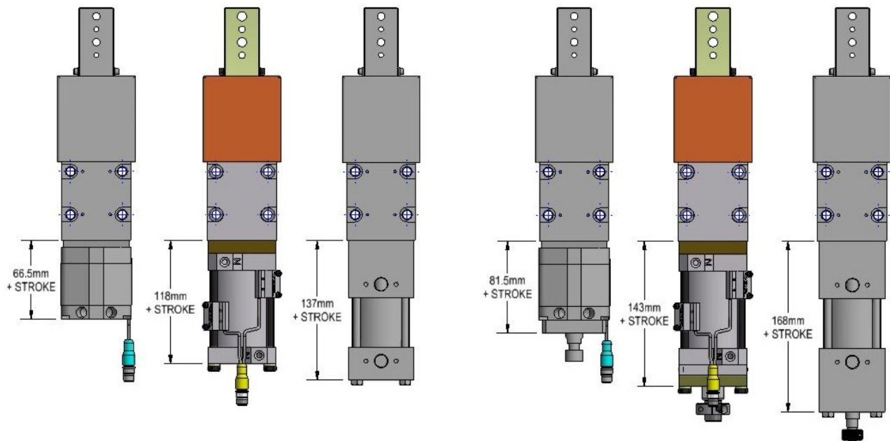
Single rod shown, 25mm stroke
